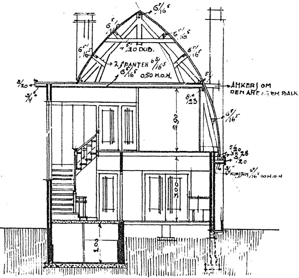
DOORSNED
