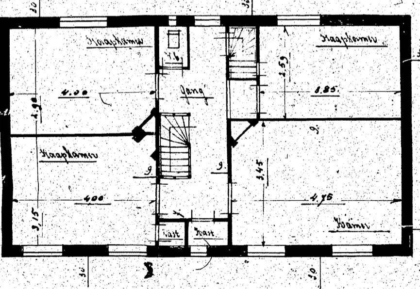
Plan Vindering
