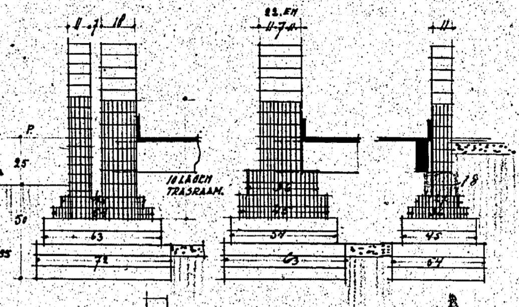
FUNDERING DETAIL? SCHAAL 1:20
